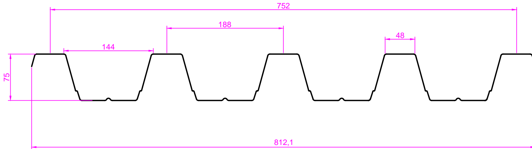
75-750 BETON ALTI TRAPEZ SAC 750 mm KAPATIR
